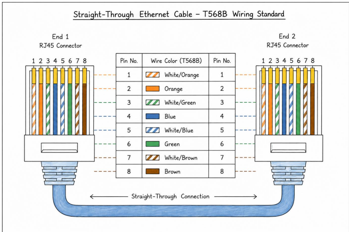
Figure : Internal Wiring of a Straight-Through Ethernet Cable (T568B Wiring Standard).
